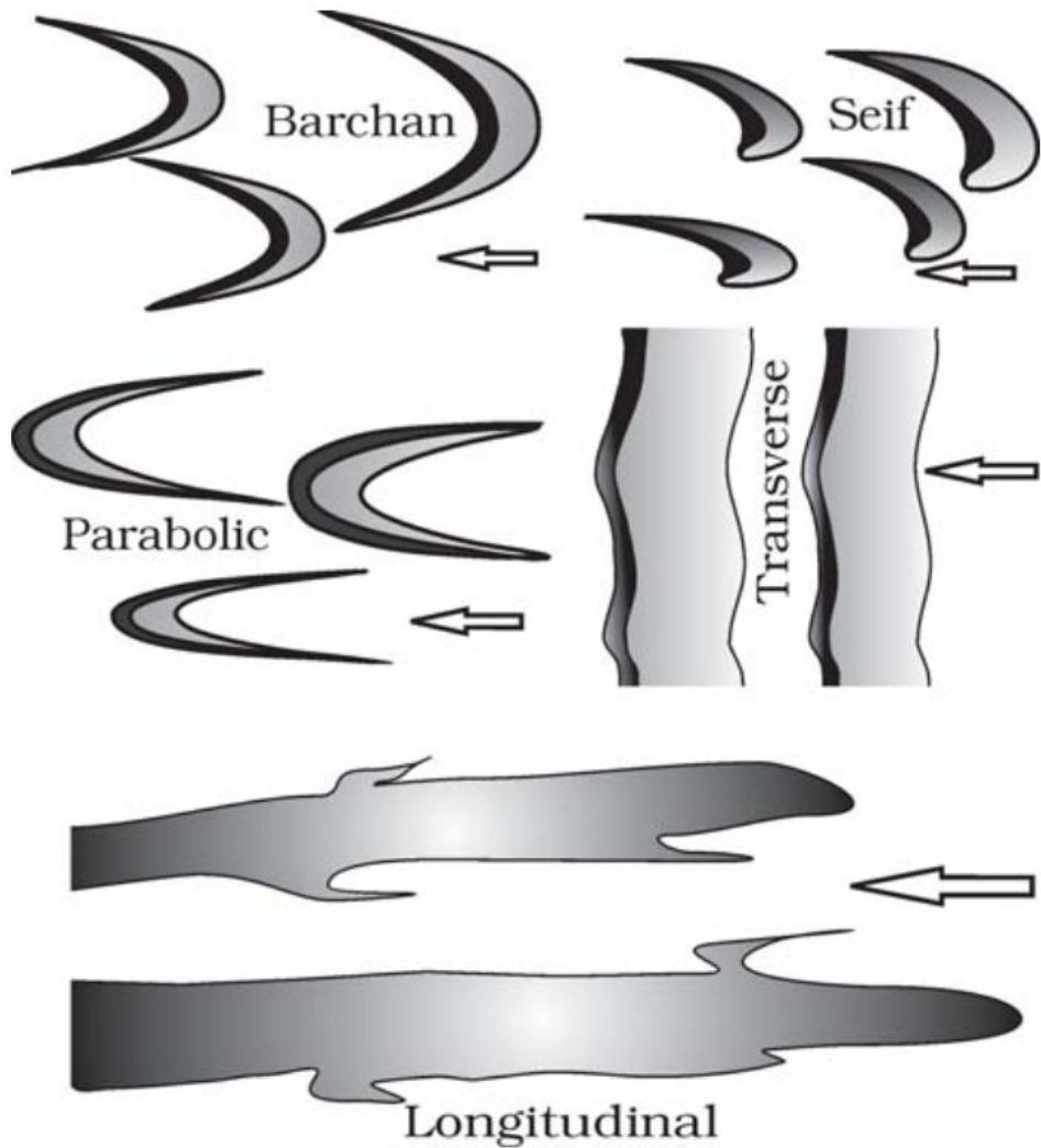
Various types of sand dunes Arrows indicate wind direction
