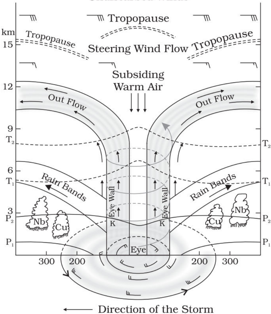
Vertical section of the tropical cyclone (after Rama Sastry)
