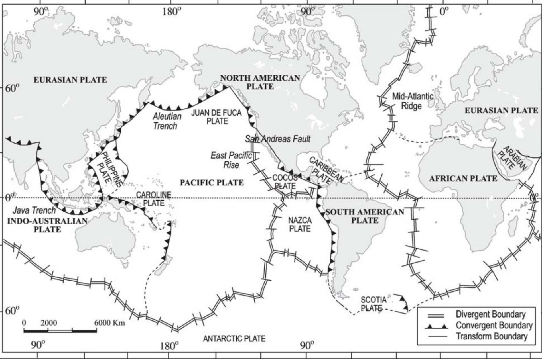
Major and minor plates of the world
