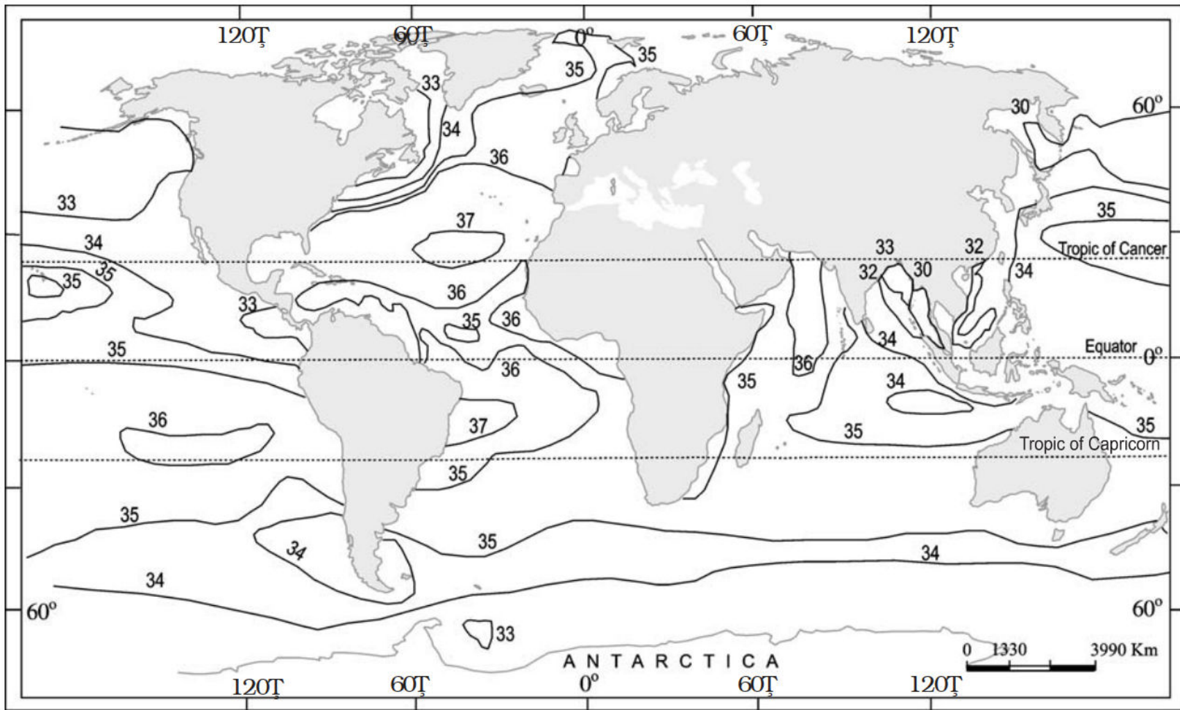
Surface salinity of the World's Oceans
