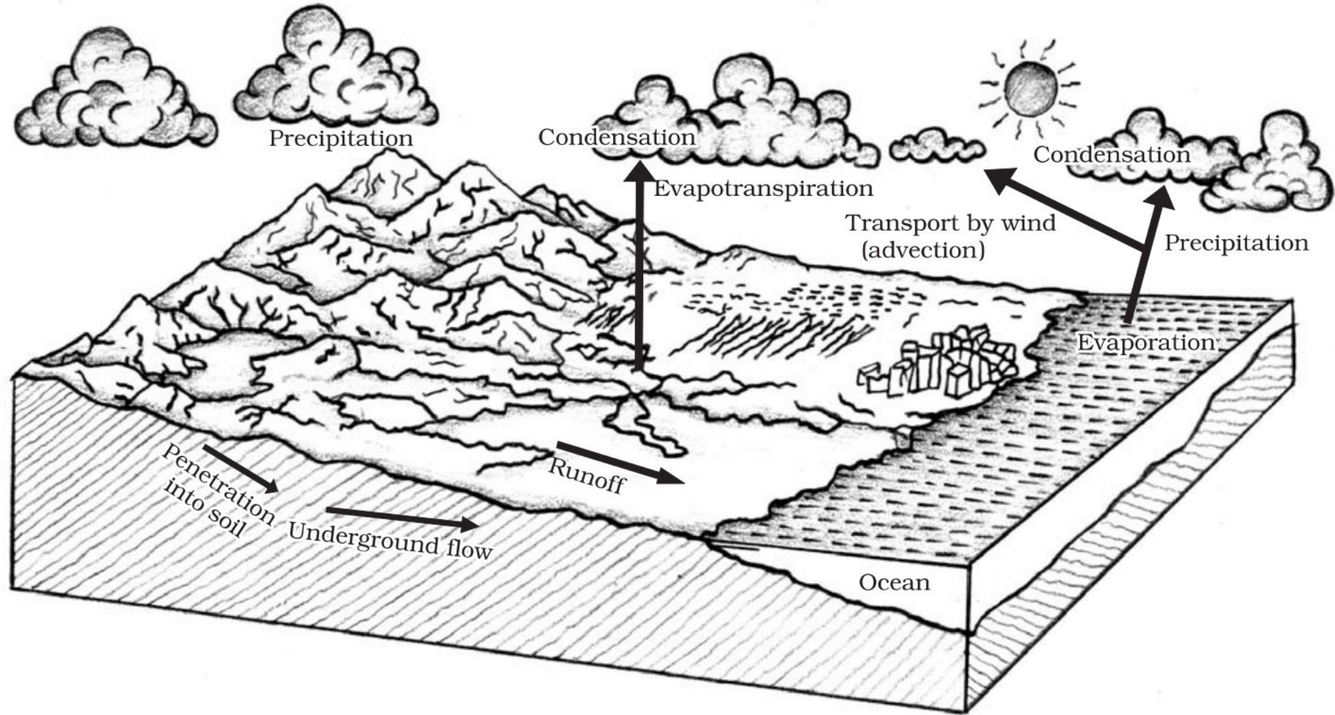
Hydrological Cycle
