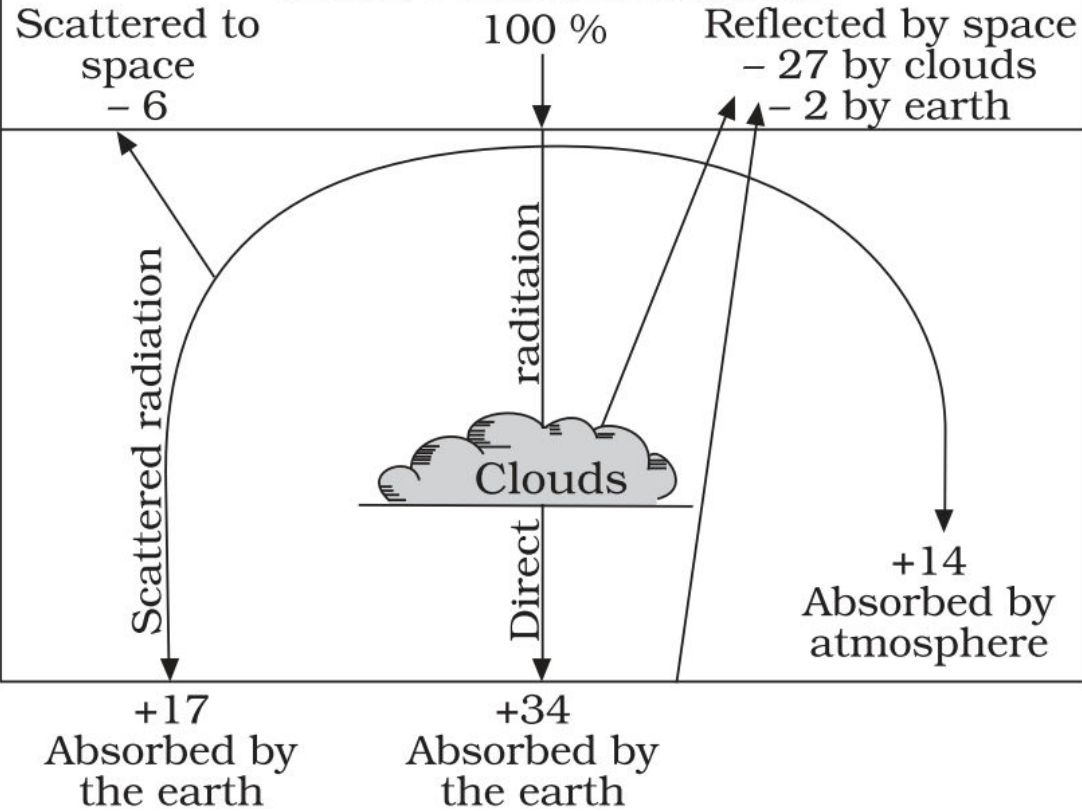
Heat budget of the earth
