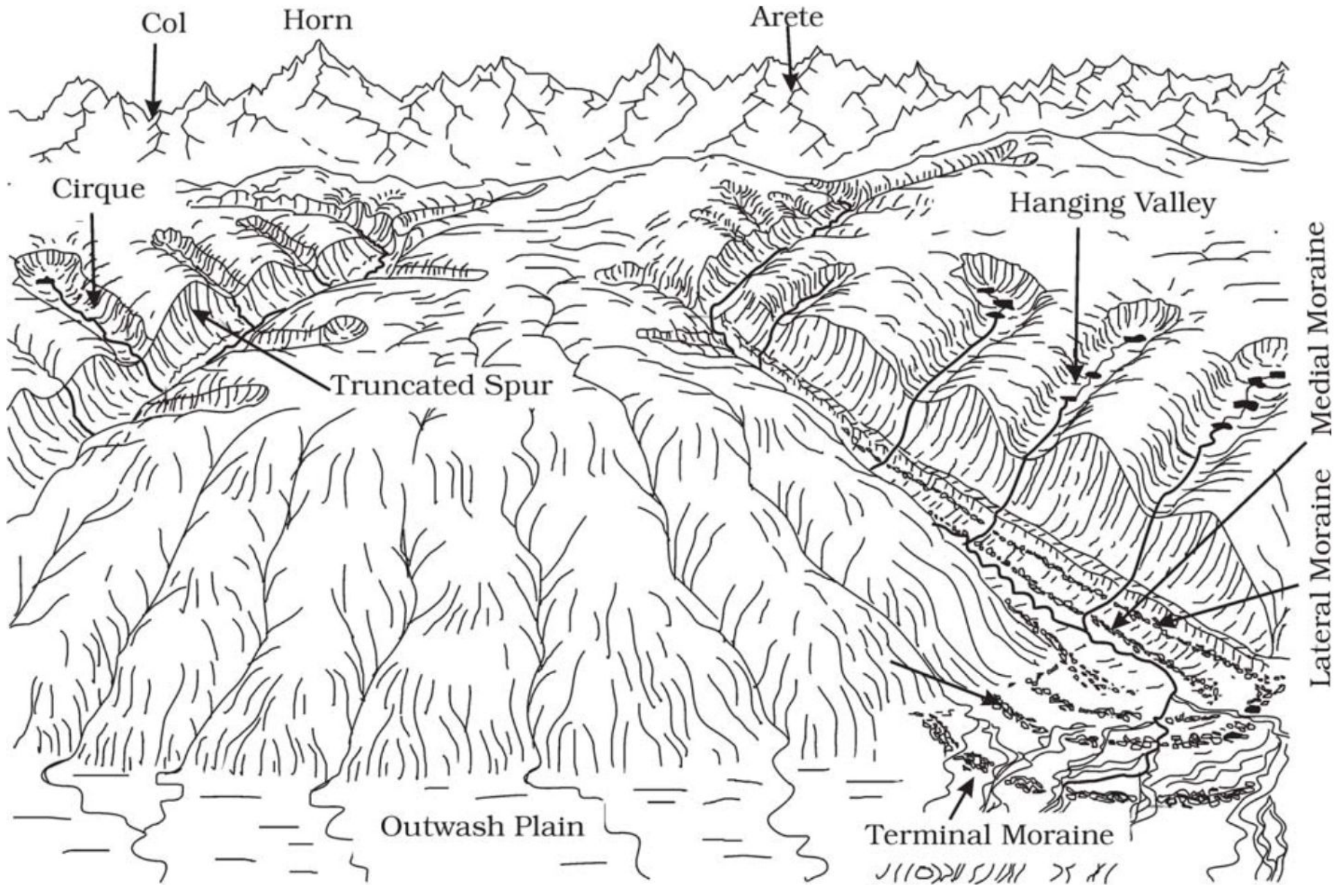
Some glacial erosional and depositional forms (adapted and modified from Spencer, 1962)
