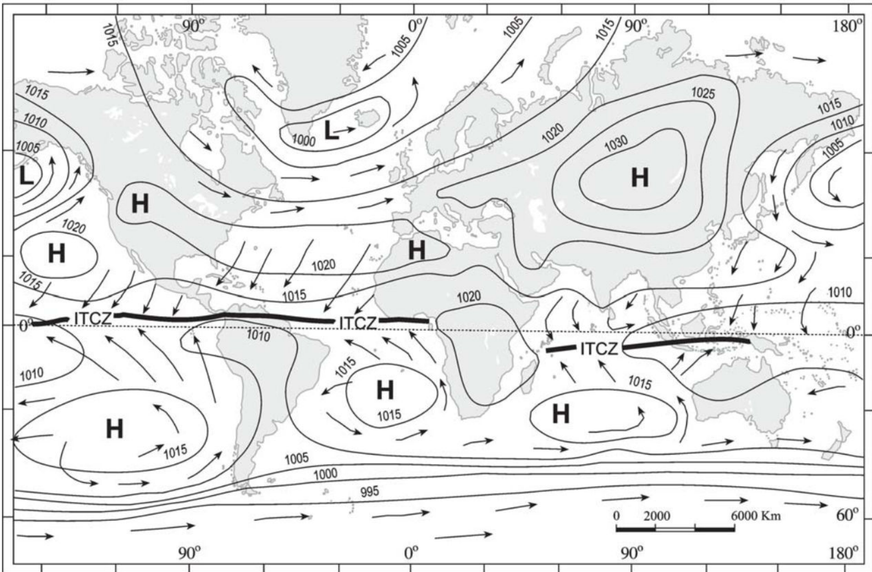
Distribution of pressure (in millibars) — January
