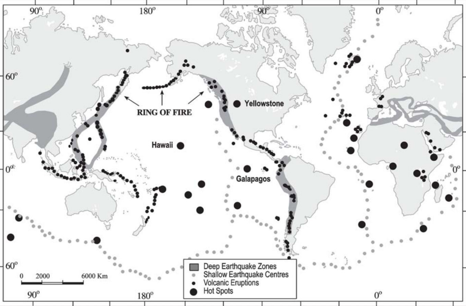
Distribution of earthquakes and volcanoes
